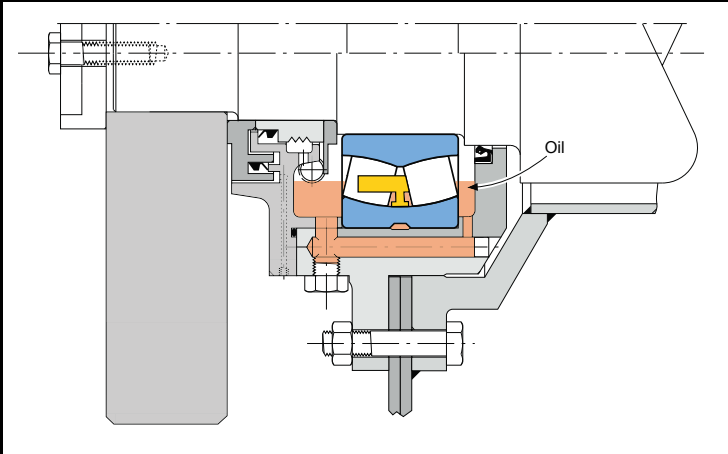
Example of ZKL spherical roller bearing vibration applications
