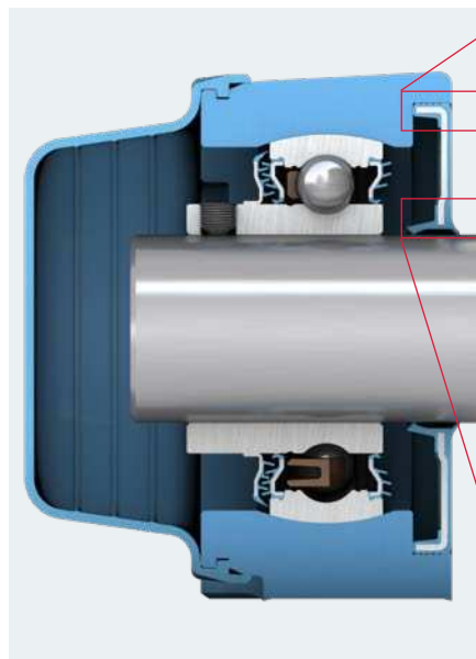
Oval flanged
