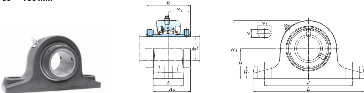
XDS2SN Cylindrical bore (with set screw collar lock (both)) d 60 ~ 100 mm
