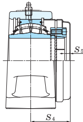
Pressed Steel Cover with ZS Unit
