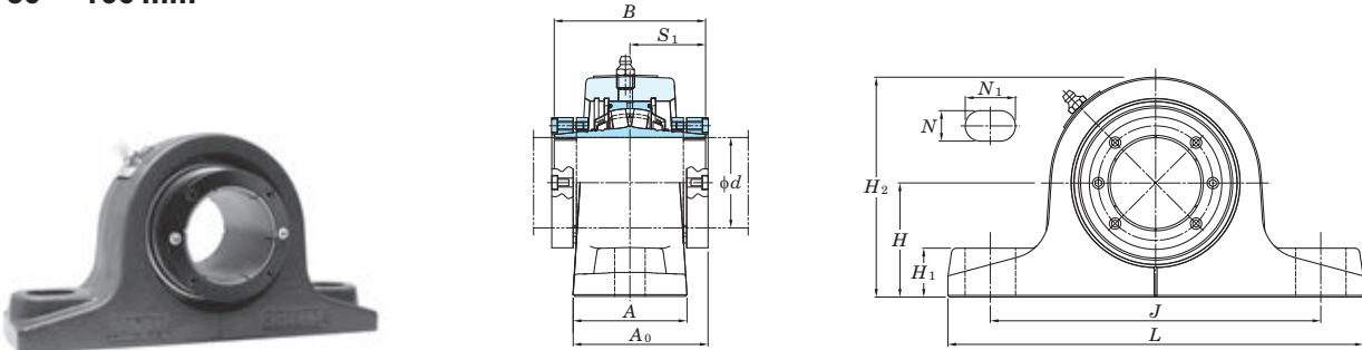
ZDS2SN Cylindrical bore (with Z-LOCK (both)) d 60 ~ 100 mm
