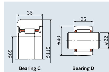
Fig. 5 Test bearings
