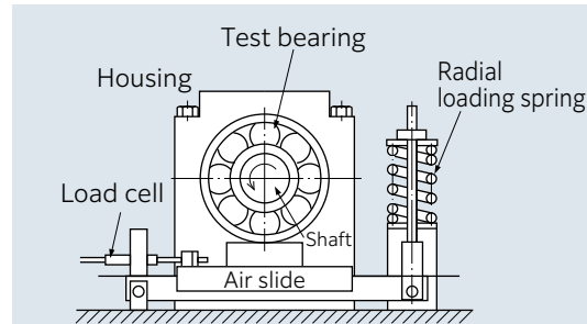
Fig. 3 Rotational torque test equipment
