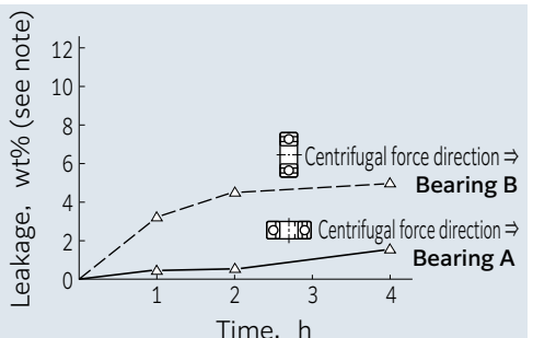
Fig. 2 Lubricant leakage test results
