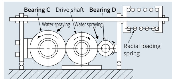
Fig. 4 Salt water test equipment
