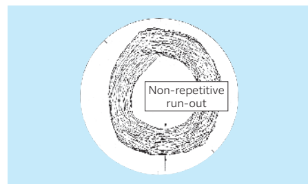
Fig. 2.3 Lissajous figure
