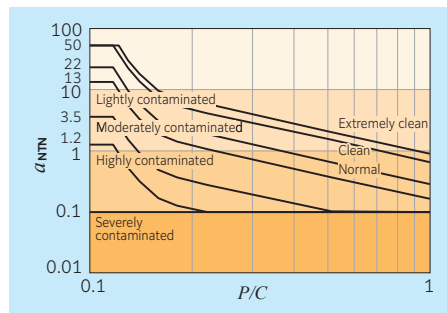
Fig. 3.6 Correlation between P/C and a_{NTN} (effect of foreign matter in roller bearing)
