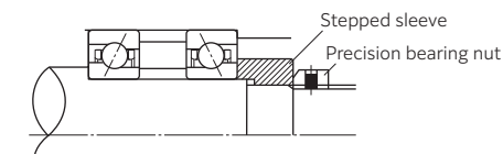
Fig. 6.8 Clamp with stepped sleeve + precision bearing nut
