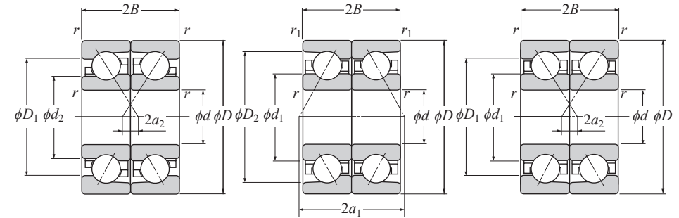
Face-to-face (DF) Drawings 1
