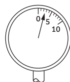
Fig. 6.25 Reading on dial gauge: +2.5 \mu\text{m} (mounted internal clearance: +1 \mu\text{m} )
