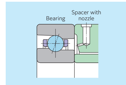
Fig. 7.3 Feed system for air-oil lubrication
