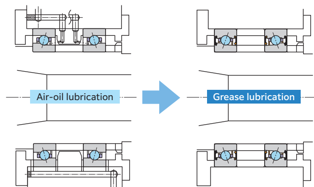
Fig. 9.44 Modification of lubrication system (air-oil lubrication to grease lubrication)
