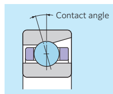
Fig. 9.1 Contact angle
