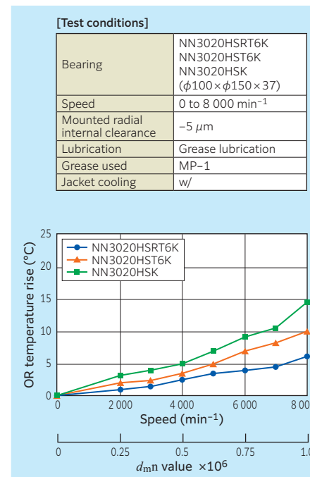
Fig. 10.5 Operation test results (grease lubrication with jacket cooling)
