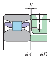
Fig. 7.10 N10HSR types
