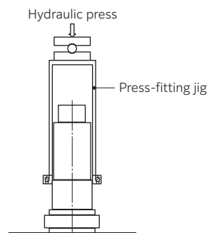
Fig. 6.1 Press-fitting pressure
