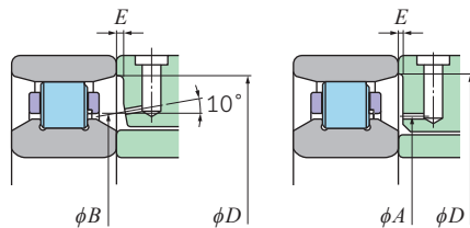
Fig. 7.9 N10HS types
