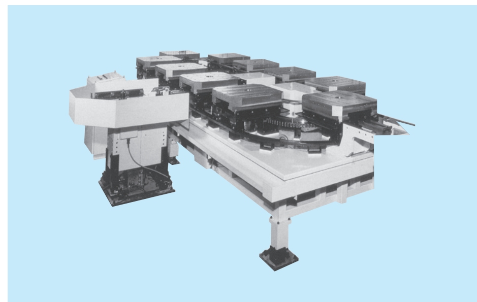
Example application of NTN cam followers for pallet changer (Photo: courtesy of Tsudakoma Corporation)
