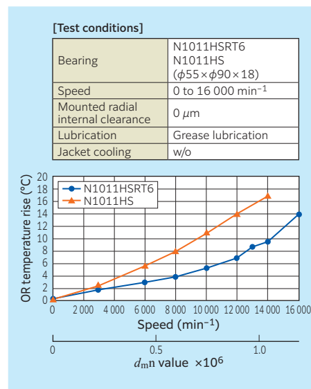
Fig. 10.11 High speed test results (grease lubrication without jacket cooling)
