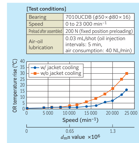
Fig. 9.23 High speed test with air-oil lubrication
