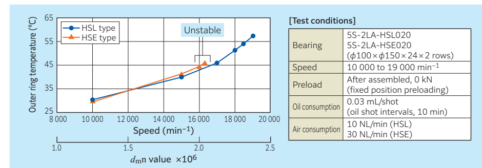
Fig. 9.33 High speed test results (fixed position preloading)
