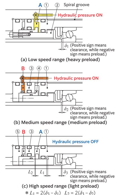
Fig. 5.3 Operating mechanism of adjustable preload
