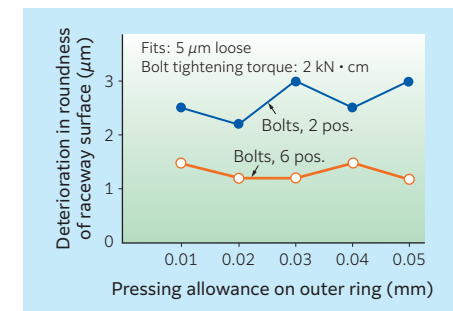
Fig. 6.15 Pressing allowance on outer ring vs. deterioration in roundness of raceway surface
