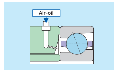
Fig. 9.21 79U and 70U types
