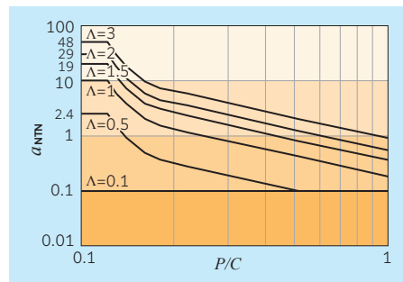
Fig. 3.8 Correlation between P/C and a_{NTN} (effect of \Lambda with roller bearing)
