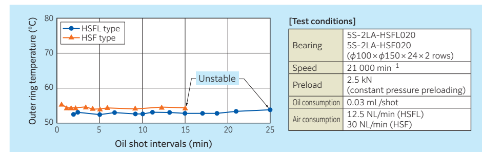
Fig. 9.32 Relationship between oil shot intervals and temperature rise
