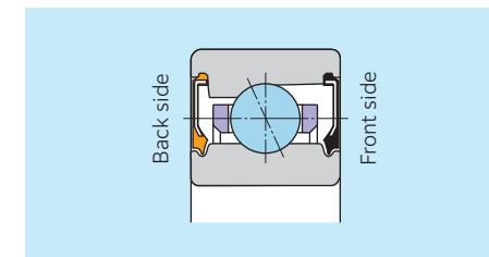
Fig. 9.39 79 LLB and 70 LLB types
