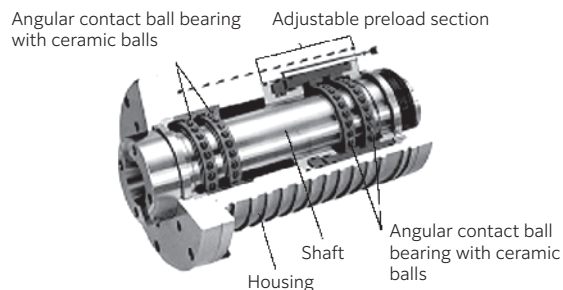
Fig. 5.1 Typical spindle configuration incorporating adjustable preload bearing unit
