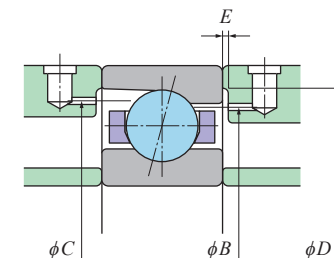
Fig. 7.7 70C and 72C types
