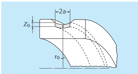
Fig. 3.1 Stress volume resulting from rolling contact according to L-P theory
