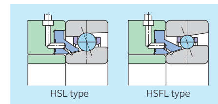
Fig. 9.5 Eco-friendly angular contact ball bearings
