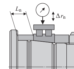
Fig. 6.20 Clearance measurement after insertion of spacer
