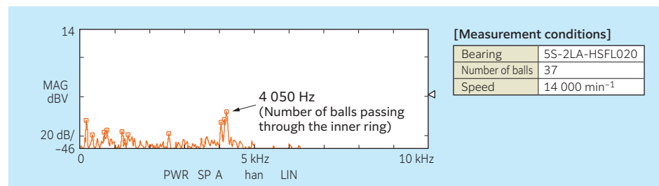
Fig. 8.13 Bearing noise frequency analysis results (Eco-friendly nozzle)
