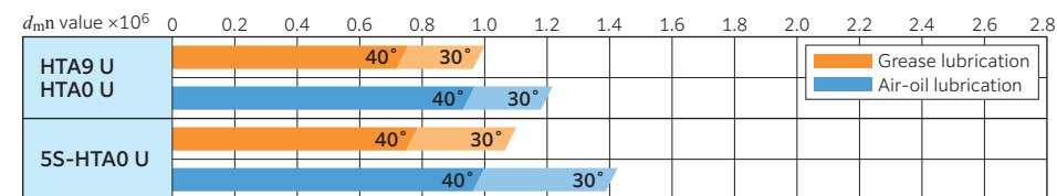
Fig. 11.2 HTA U type
