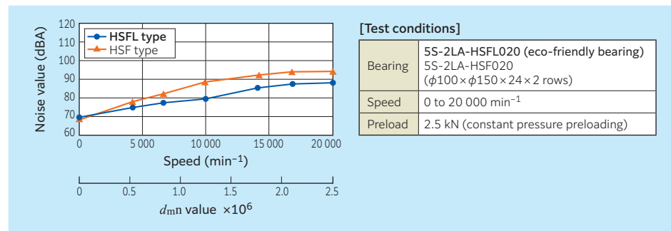
Fig. 8.11 Comparison of noise values
