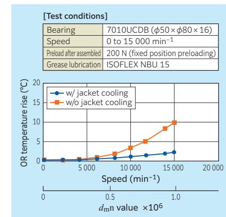
Fig. 9.22 High speed test with grease lubrication
