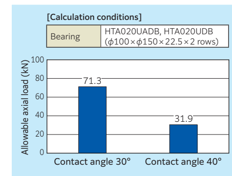
Fig. 11.4 Comparison of allowable axial load
