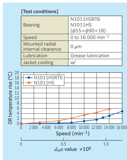
Fig. 10.12 High speed test results (grease lubrication with jacket cooling)
