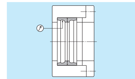
Fig. 6.13 Measuring position for roundness on outer ring raceway surface
