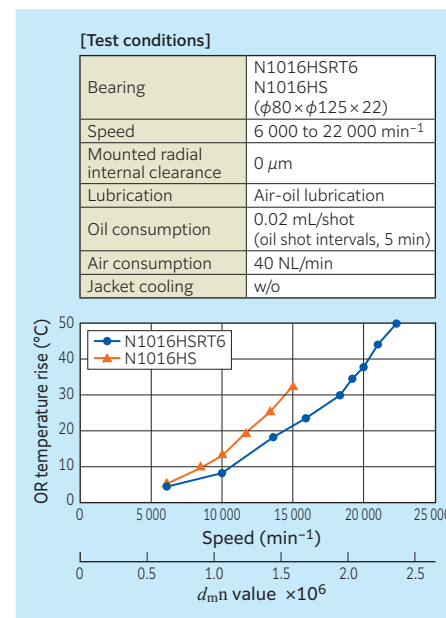
Fig. 10.13 High speed test results (air-oil lubrication without jacket cooling)
