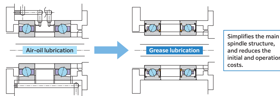
Fig. 9.40 Modification of lubrication system (air-oil lubrication to grease lubrication)
