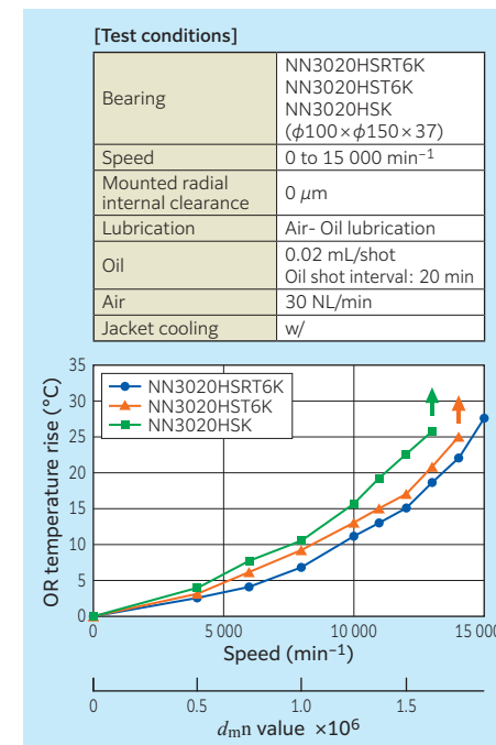
Fig. 10.6 Operation test results (air-oil lubrication with jacket cooling)
