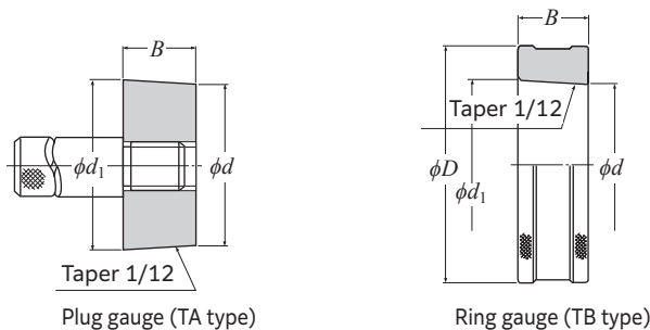
Dimension table for taper gauge
