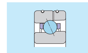
Fig. 9.6 Air-oil lubricated high speed angular contact ball bearings with re-lubricating hole on the outer ring
