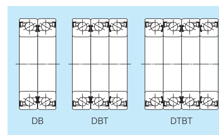
Fig. 13.2 Bearing arrangement
