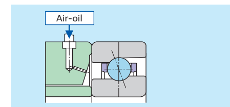
Fig. 8.7 Standard nozzle
