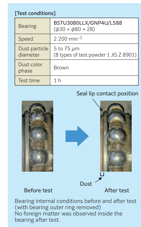
Fig. 13.15 Dust test results
