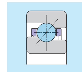
Fig. 11.2 HTA U type
