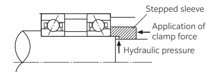
Fig. 6.7 Clamp with stepped sleeve
