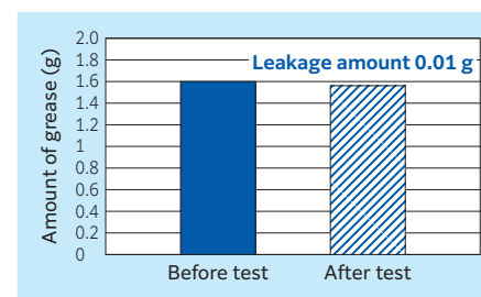
Fig. 13.9 Grease leakage
