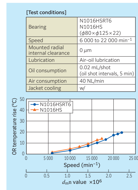
Fig. 10.14 High speed test results (air-oil lubrication with jacket cooling)
