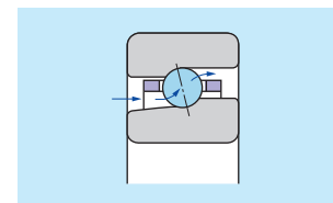
Fig. 9.4 Ultra high speed angular contact ball bearings
