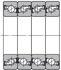
When three rows bear axial load (DBTT)
