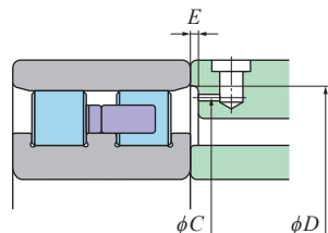
Fig. 7.8 NN30 and NN30T6 types
