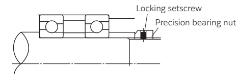
Fig. 6.9 Clamp with precision bearing nut
