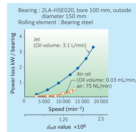
Fig. 7.12 Comparison of power loss with air-oil lubrication and with jet lubrication
