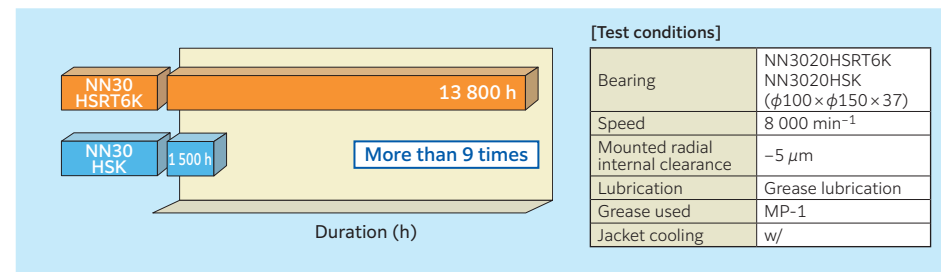
Fig. 10.7 Durability test results
