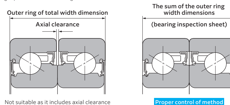
Fig.13.22 Outer ring width control of face-to-face duplex BST type
