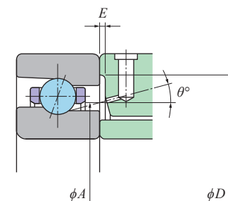
Fig. 7.5 BNT and HTA U types
