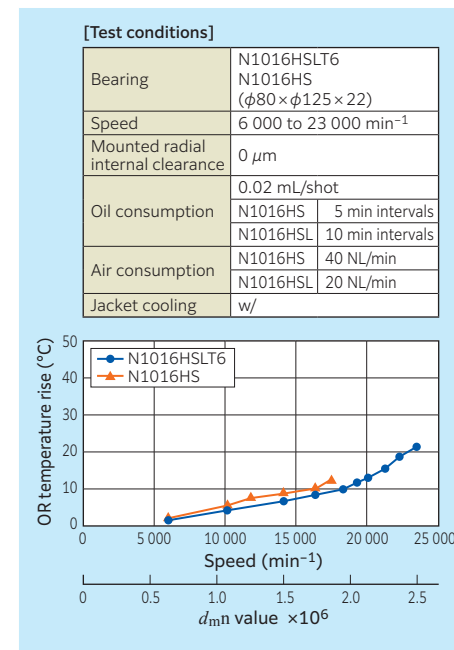
Fig. 10.17 High speed test results (with Jacket cooling)
