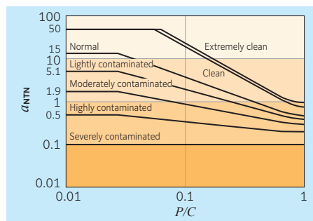
Fig. 3.5 Correlation between P/C and a_{NTN} (effect of foreign matter in ball bearing)
