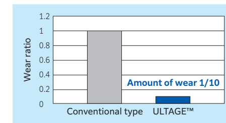
Fig. 13.6 Ratio of fretting corrosion while rolling
