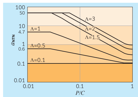
Fig. 3.7 Correlation between P/C and a_{NTN} (effect of \Lambda with ball bearing)
