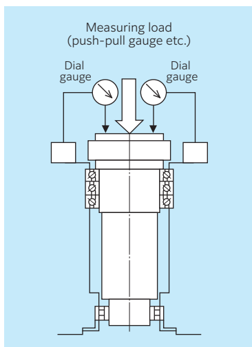
Fig. 6.16 Checking for axial rigidity
