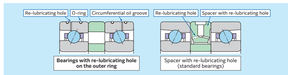
Fig. 9.34 HSEW type
